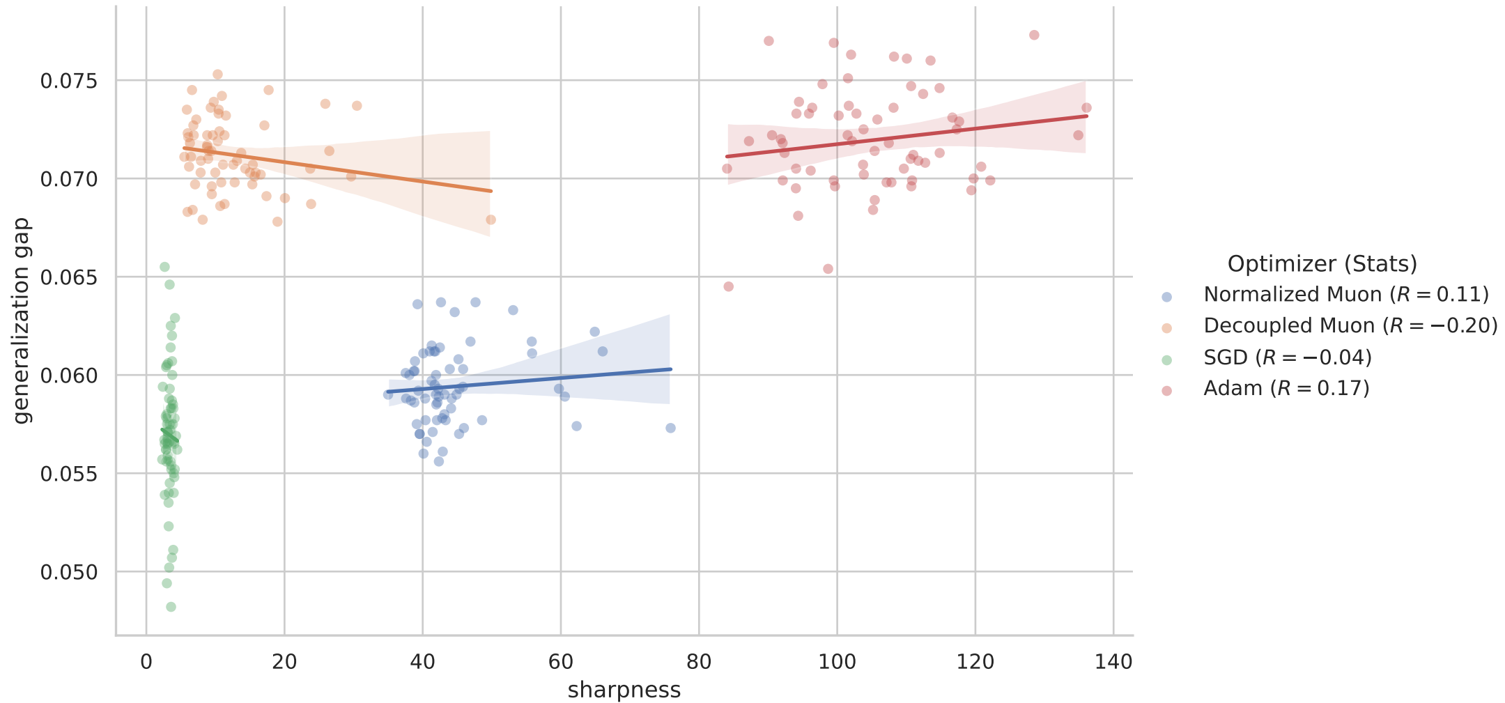
Correlation: sharpness vs generalization gap
